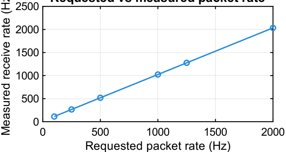
Requested vs measured packet rate
